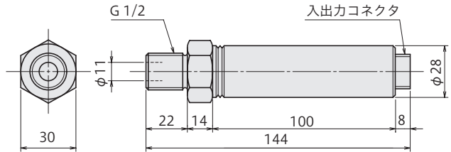
PWH-70/-100MPa
