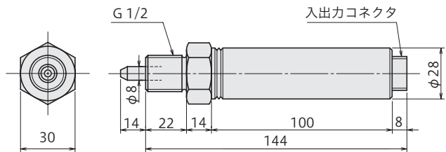
PWH-150/-200MPa
