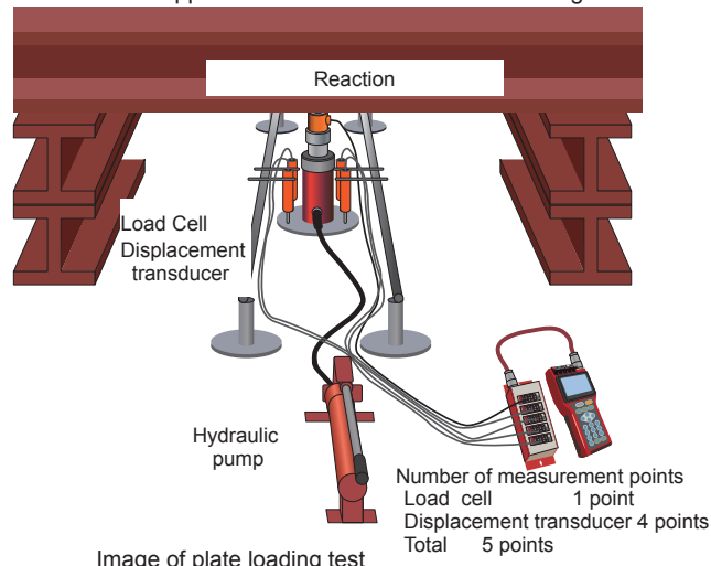
Image of plate loading test
