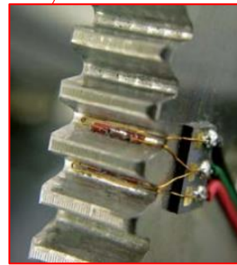
Static Strainmeters
