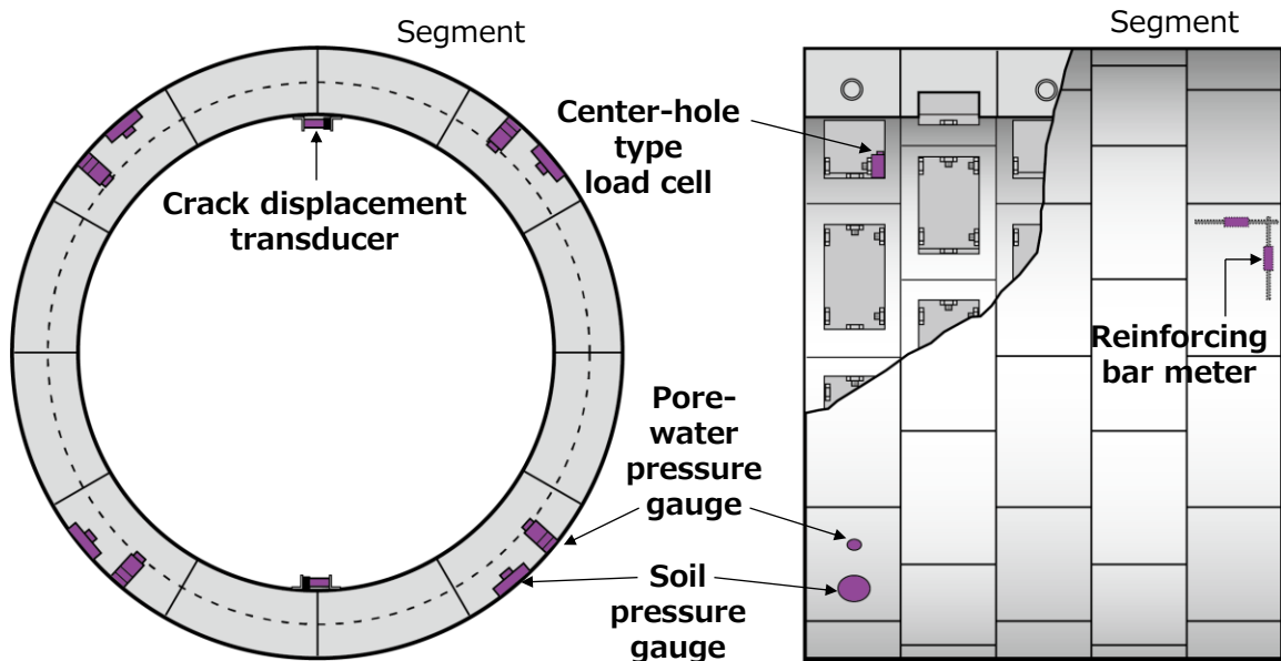
[ Measuring System Block Diagram ]
