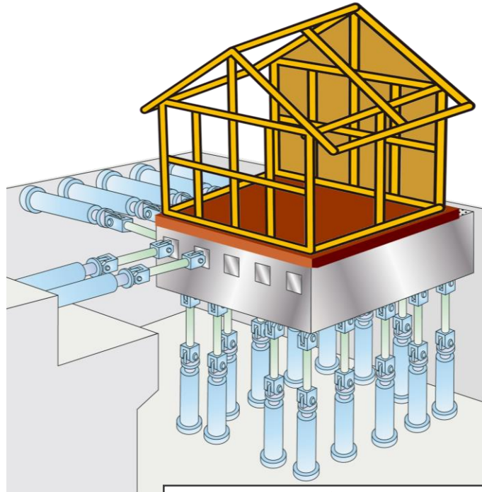
Full-scale three-dimensional vibration table
